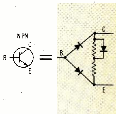
Fig. 1 Equivalent circuit of an NPN transistor shows three interconnected diodes which represent the relationships of the three elements of a transistor—emitter, base, collector. For the PNP type, polarity of the diodes would be reversed.
