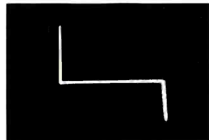
Fig. 6 Curve produced on a solid state scope as a result of protective zener action in the horizontal sweep circuit of the scope. Many scopes will overload when the collector voltage control is set to produce higher voltages. False curves can be the result.
