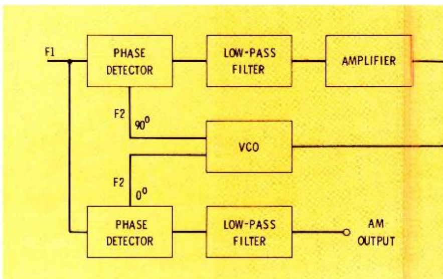
Fig. 4 Special circuit designed to demodulate AM with a phase-locked loop.
