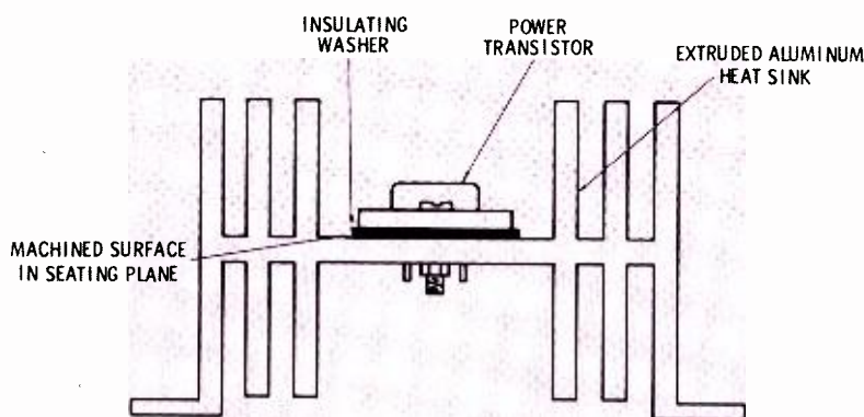
Fig. 2a Power transistor with heat sink and necessary thermal hardware.
